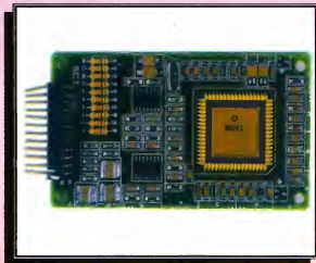
This is the chip that makes the 3-D sound possible in the NuReality system.
